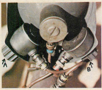
U.S. M3 infrared sniper scope from rear. Knob on left (A) controls electronic focusing of telescope while knob on right (B) allows varying intensity of reticle; consists of small vertical bar of light that appears in field of view. Can be turned off for surveillance and, via rheostat, made progressively brighter for actual sniping work. Center cable (with blue connector) provides power to operate 30-watt IR light source.
